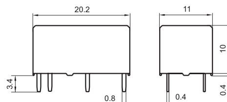
2 coils latching
