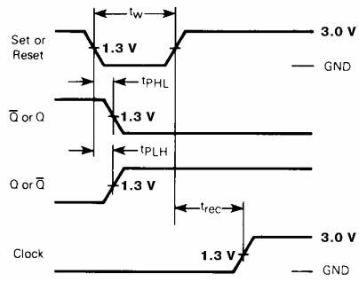
Figure 2. Switching Waveforms
