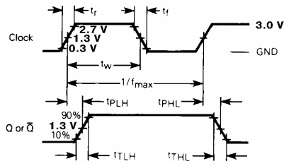
Figure 1. Switching Waveforms
