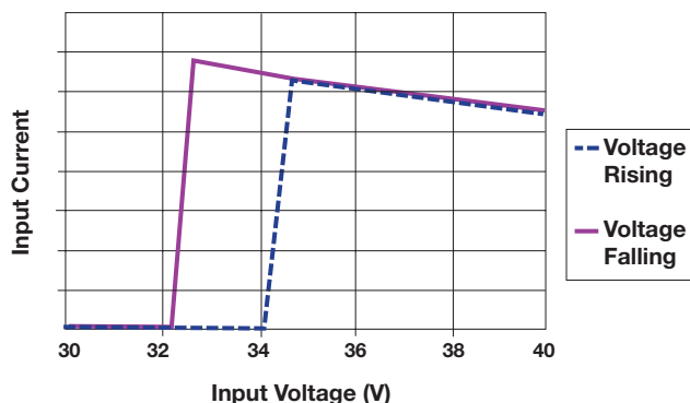
Undervoltage Lockout
