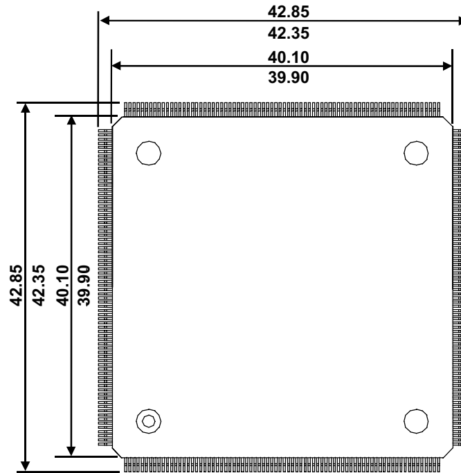
Figure 41. Physical Dimensions 1
