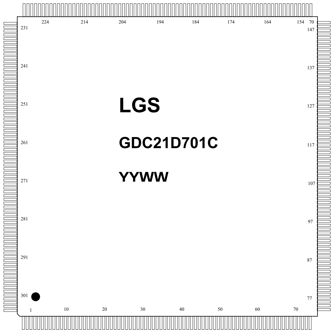
Figure 1. Pin Configuration
