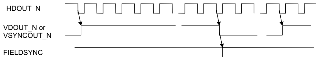
Figure 28. VSYNC Timing (Falling Edge of VDOUT_N)
