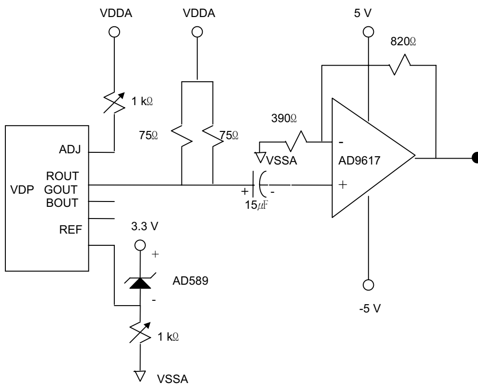
Figure 26. DAC Application Circuit
