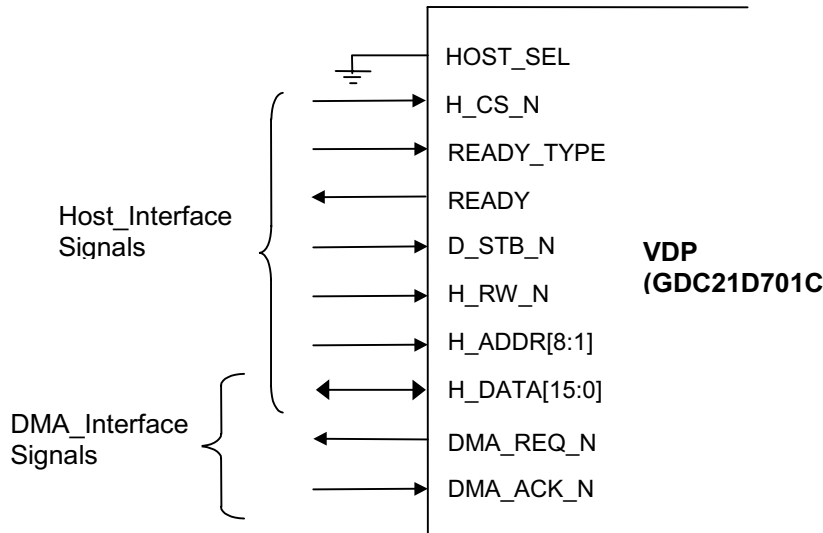
Figure 13. Host Interface
