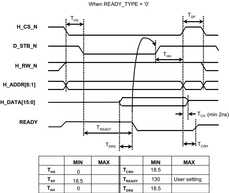
Figure 16. Host Read Timing
