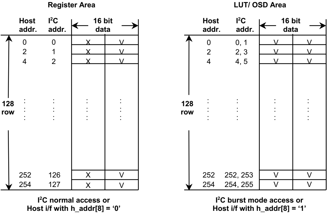
Figure 14. Address Map
