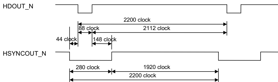
Figure 29. HSYNC Timing
