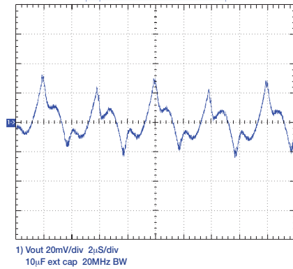
Voltage Ripple
