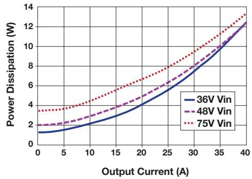
Power Dissipation
