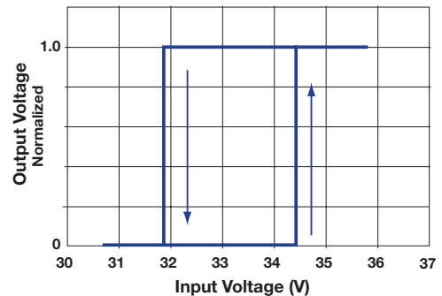
Undervoltage Hysteresis
