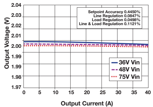
Line/Load Regulation
