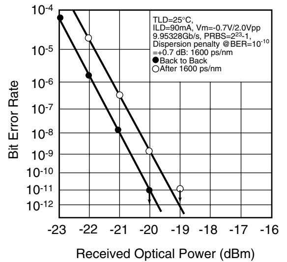
Fig. 6 Transmission Characteristics
