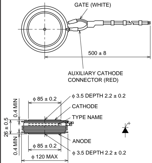
OUTLINE DRAWING
