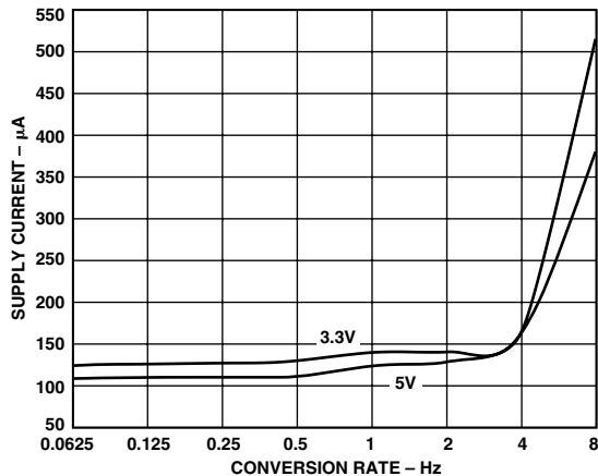
TPC 8. Operating Supply Current vs. Conversion Rate
