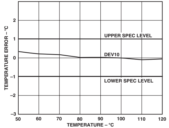
TPC 4. Temperature Error of ADM1021A vs. Pentium III Temperature
