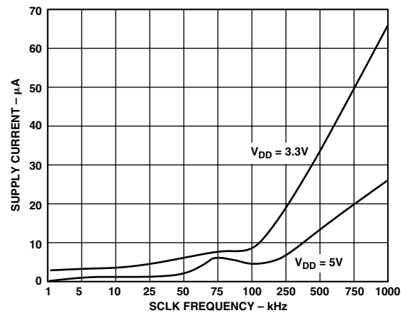
TPC 6. Standby Supply Current vs. Clock Frequency
