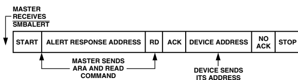
Figure 6. Use of \overline{SMBALERT}
