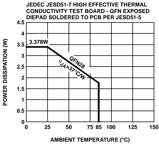
FIGURE 25. PACKAGE POWER DISSIPATION vs AMBIENT TEMPERATURE
