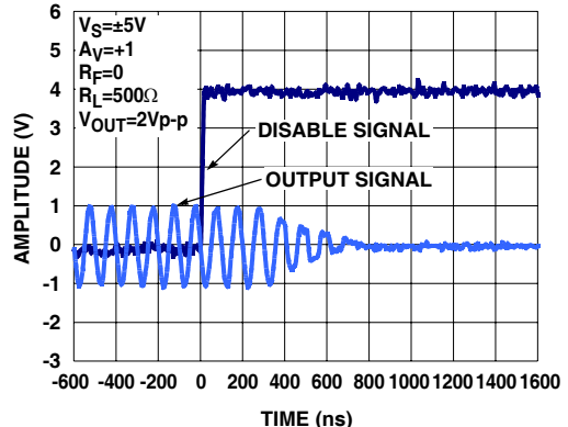
FIGURE 30. TURN-OFF TIME
