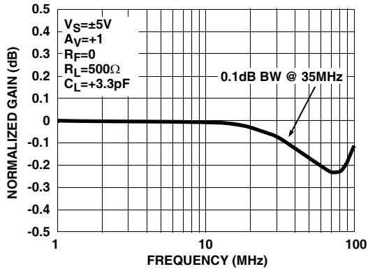
FIGURE 3. 0.1dB BANDWIDTH
