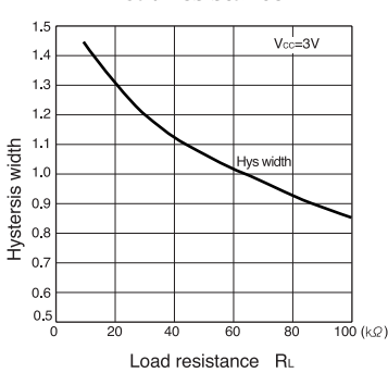
Hysteresis width Vs. Load resistance
