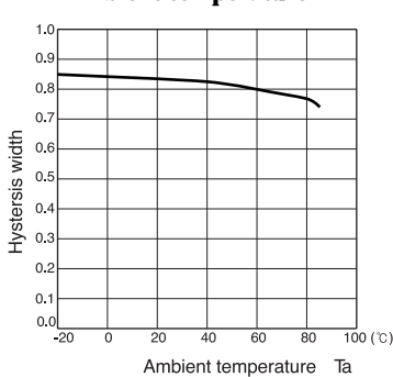
Hysteresis width Vs. Ambient temperature
