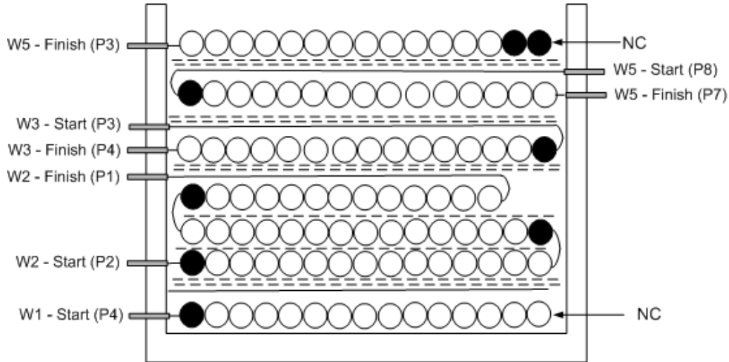
Figure 5 – Transformer Build Diagram.
