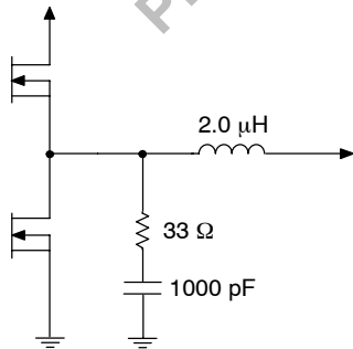
Figure 35. Filter Components
