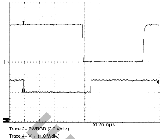
Figure 25. Power Good Response to an Out of Regulation Condition
