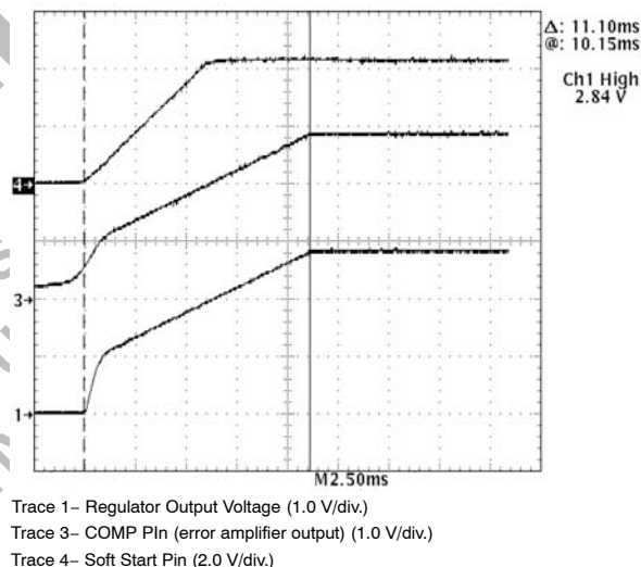
Figure 12. Demonstration Board Startup Waveforms
