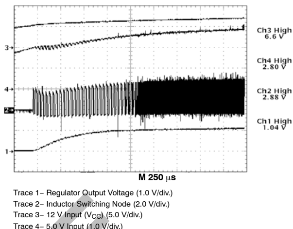
Figure 11. Demonstration Board Startup in Response to Increasing 12 V and 5.0 V Input Voltages. Extended Off Time is Followed by Normal Off Time Operation when Output Voltage Achieves Regulation to the Error Amplifier Output.
