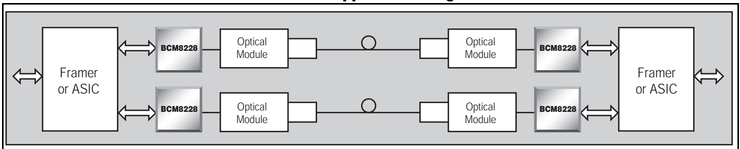
BCM8228 Application Diagram
