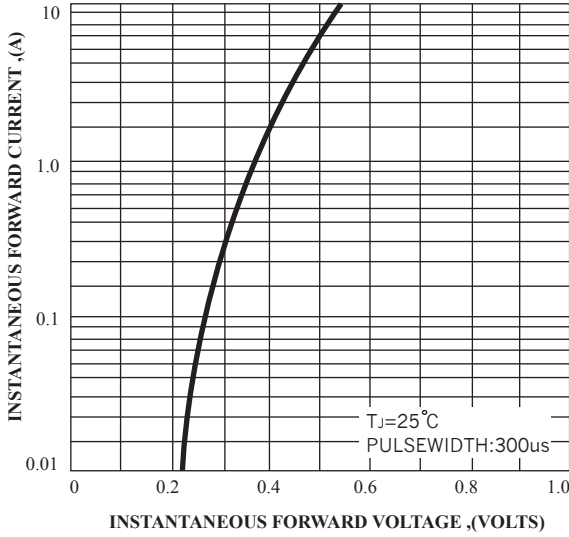
FIG.3-TYPICAL FORWARD CHARACTERISTICS
