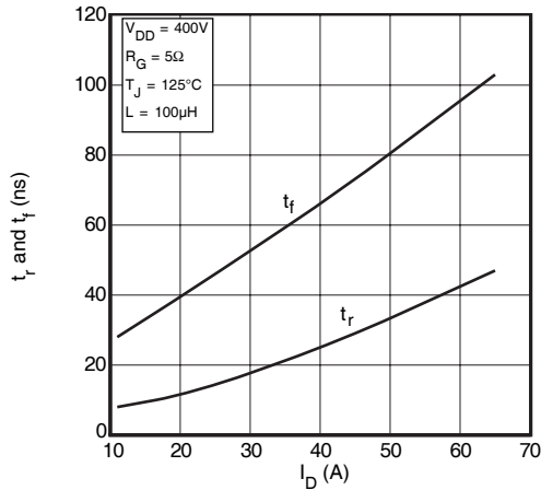
FIGURE 15, RISE AND FALL TIMES vs CURRENT
