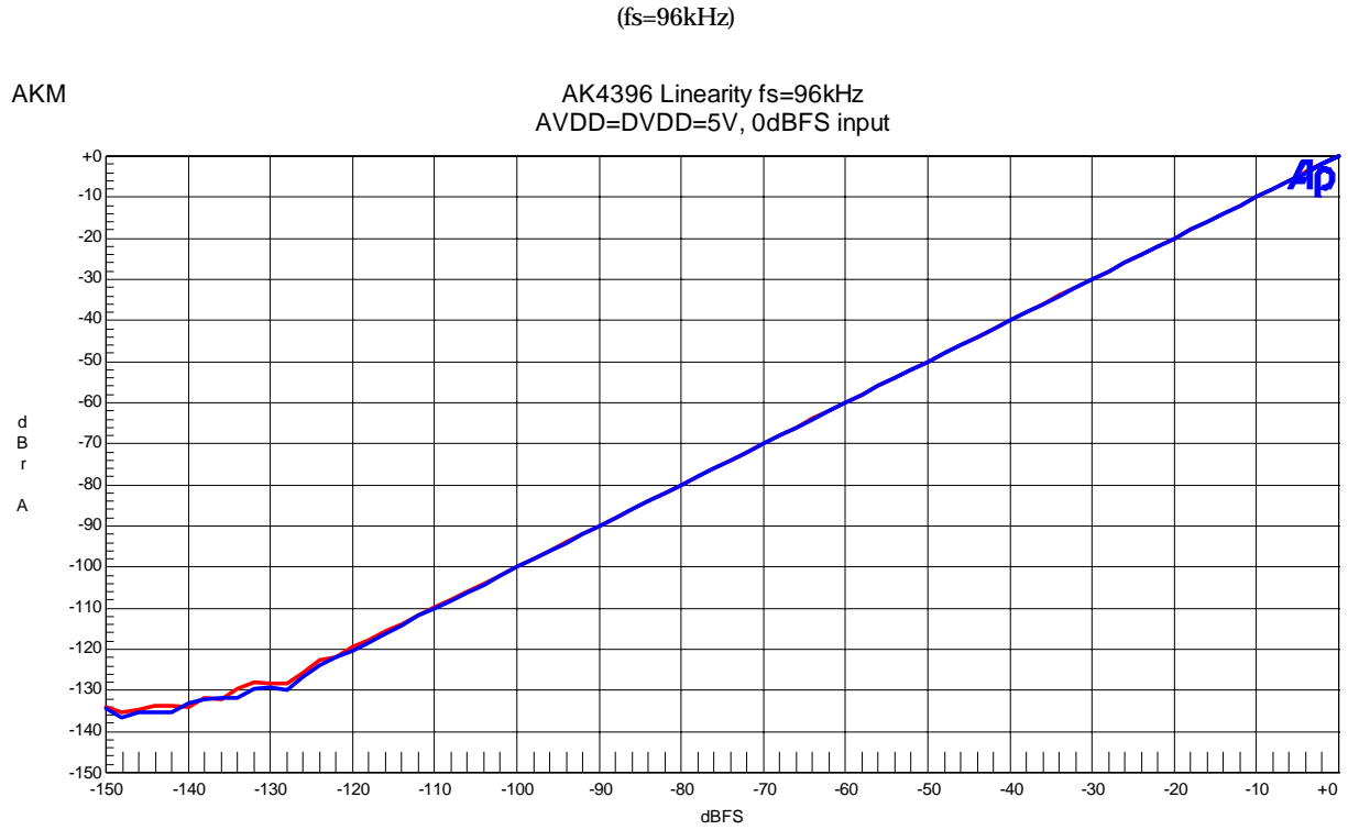
Figure 24 Linearity (fin=1kHz)
