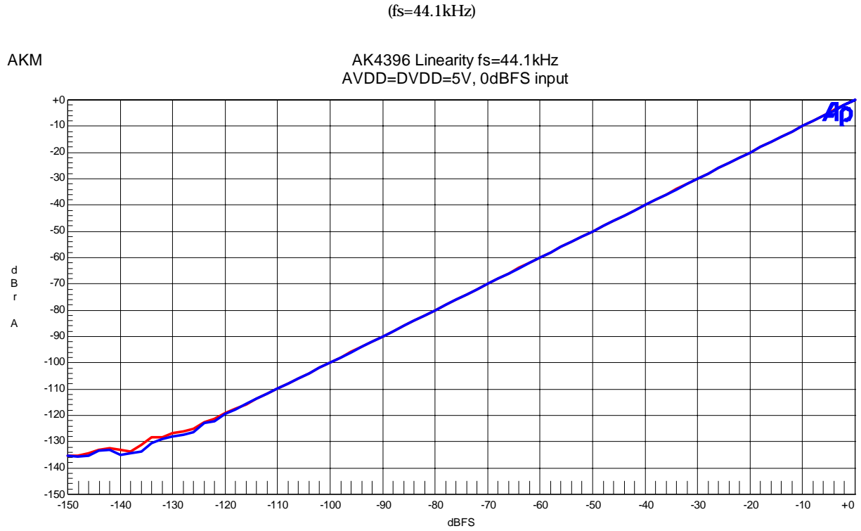
Figure 15 Linearity (fin=1kHz)
