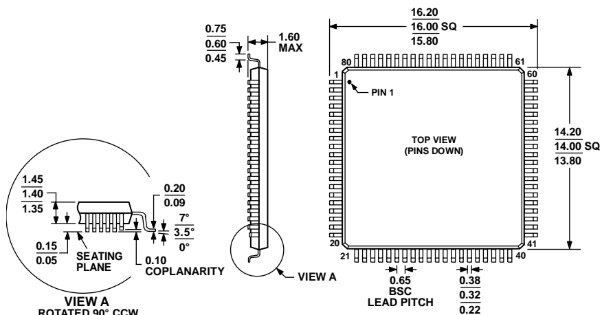
Figure 5. 80-Lead Low Profile Quad Flat Package [LQFP] (ST-80-2) Dimensions shown in millimeters
