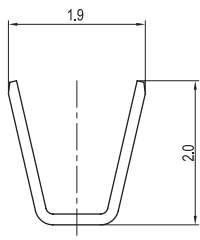
SEC D-D''
