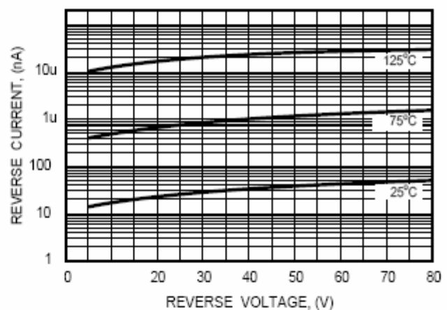
FIG. 4 - REVERSE CHARACTERISTICS
