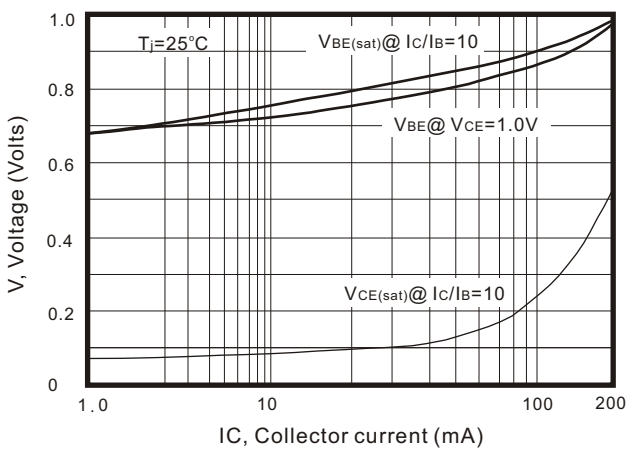
Fig. 11- "ON" voltages
