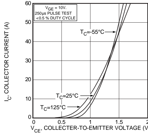
FIGURE 2, Output Characteristics ( V_{GE} = 10V )
