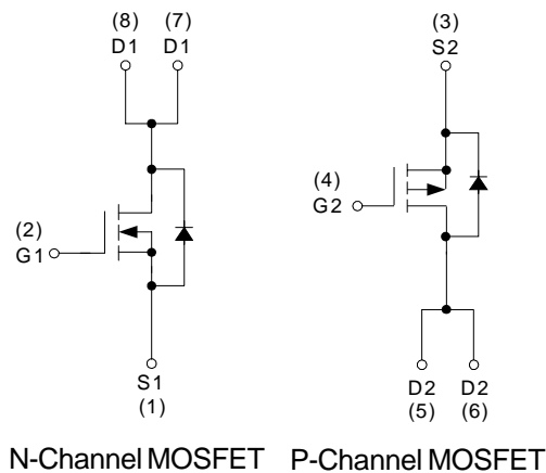
Top View of SOP – 8
