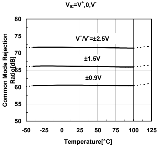
Common Mode Rejection Ratio vs. Temperature V_{IC}=V^+, 0, V^-
