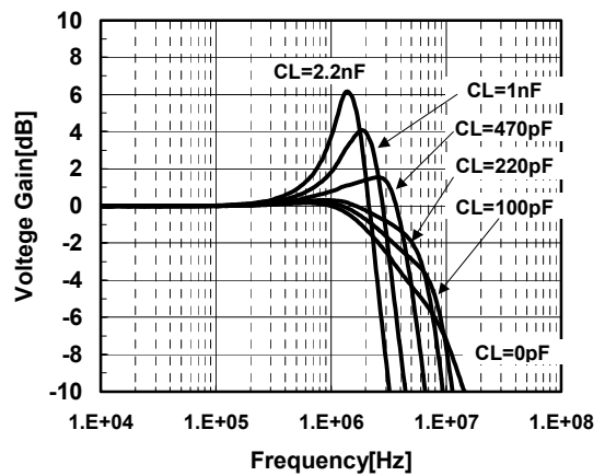
Peak Gain of Voltage Follower V^*/V=2.5V, GV=0dB R_S=50\Omega, R_L=2k\Omega, Ta=+25^\circ C
