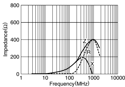
MZA2010D680C
