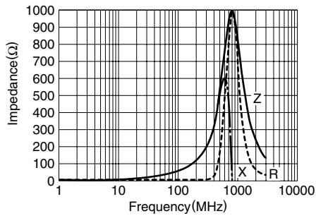
MZA2010F560C
