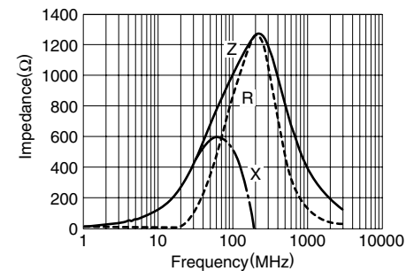
MZA2010Y102C
