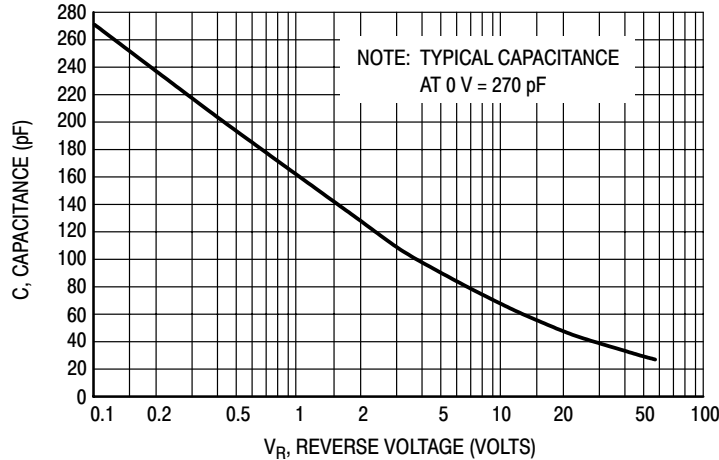
Figure 5. Typical Capacitance
