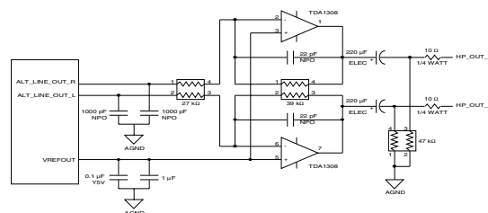
Figure 18. Stereo Output
