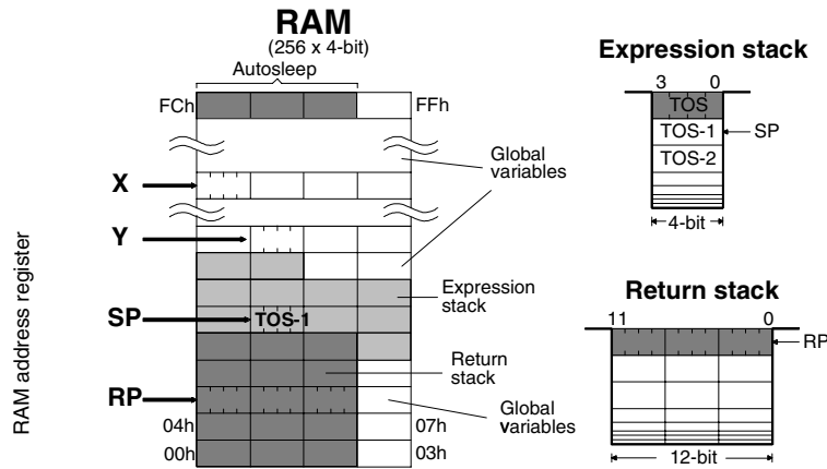
Figure 5. RAM Map
