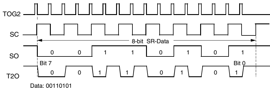
Figure 36. Bi-phase Modulation
