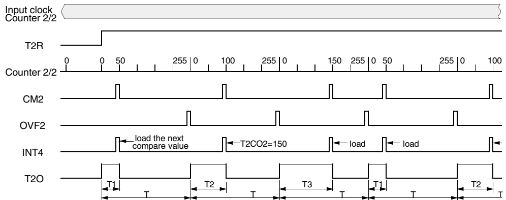
Figure 38. PWM Modulation
