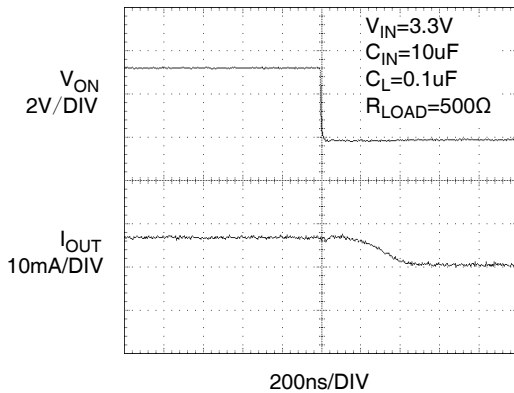
Figure 17. T_{OFF} Response
