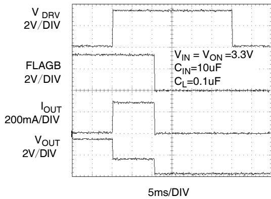
Figure 15. T_{BLANK} Response
