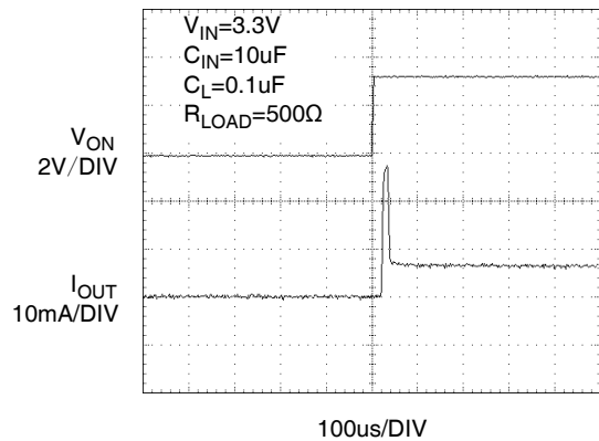
Figure 16. T_{ON} Response
