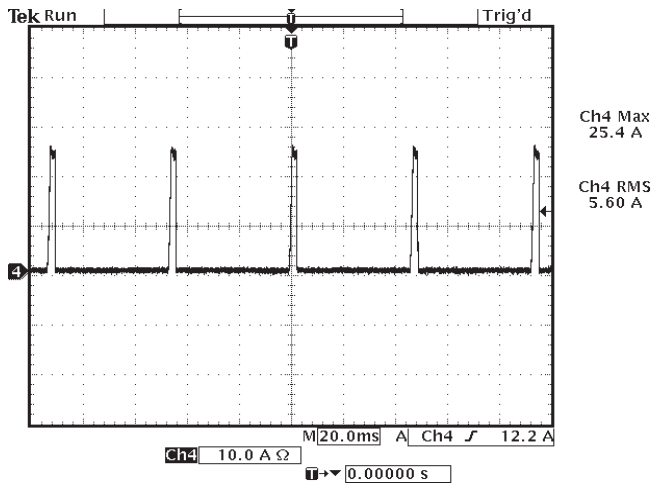
Figure 3: Short Circuit Characteristic (Channel 4: I_{s/c} )
