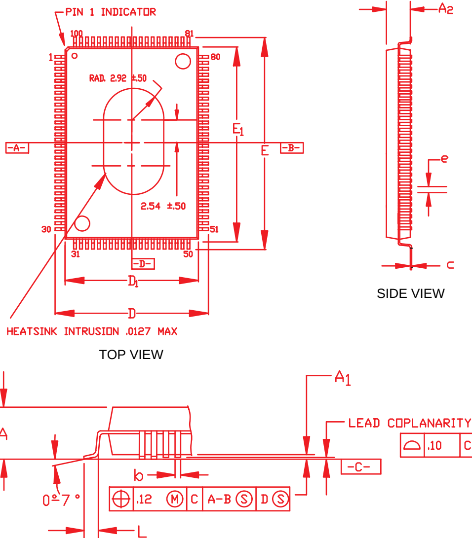
Figure 13. 100-Pin PQFP/TEP Package
