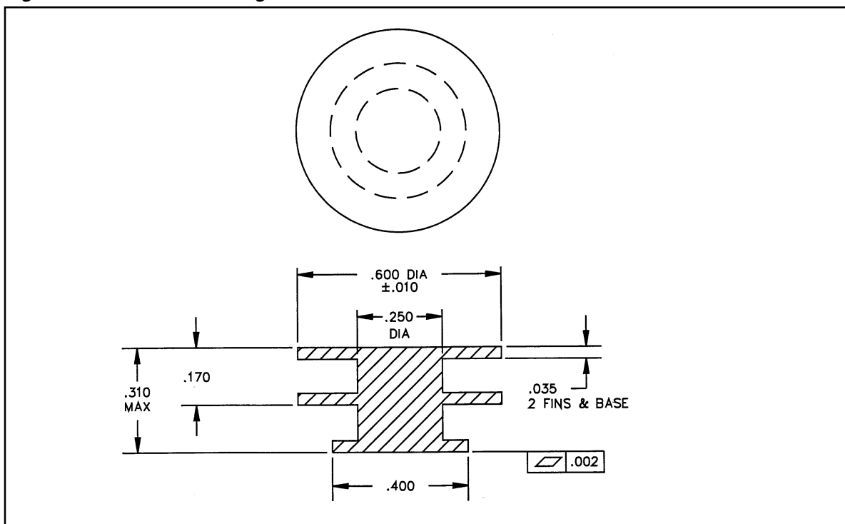
Figure 14. Heat Sink Drawing DW0045-28
