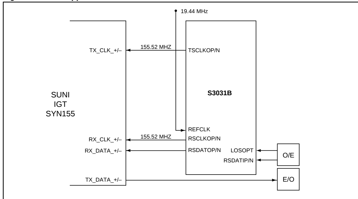
Figure 20. OC-3 Application
