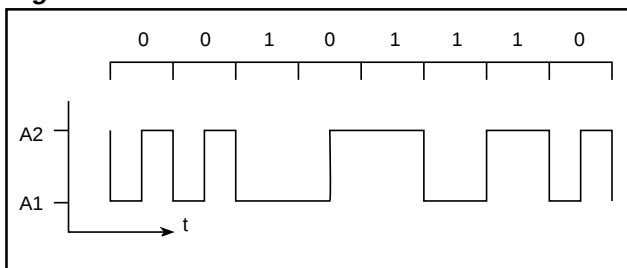
Figure 4. CMI Encoded Data
