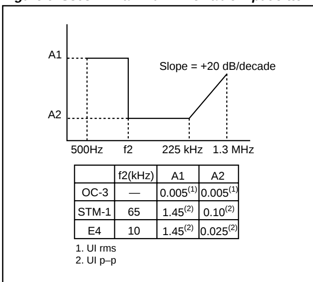
Figure 6. S3031B Maximum Allowable Input Jitter
