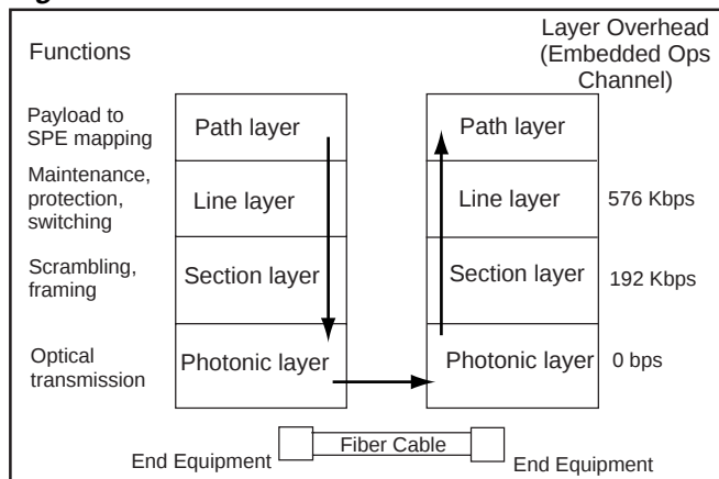
Figure 2. SONET Structure
