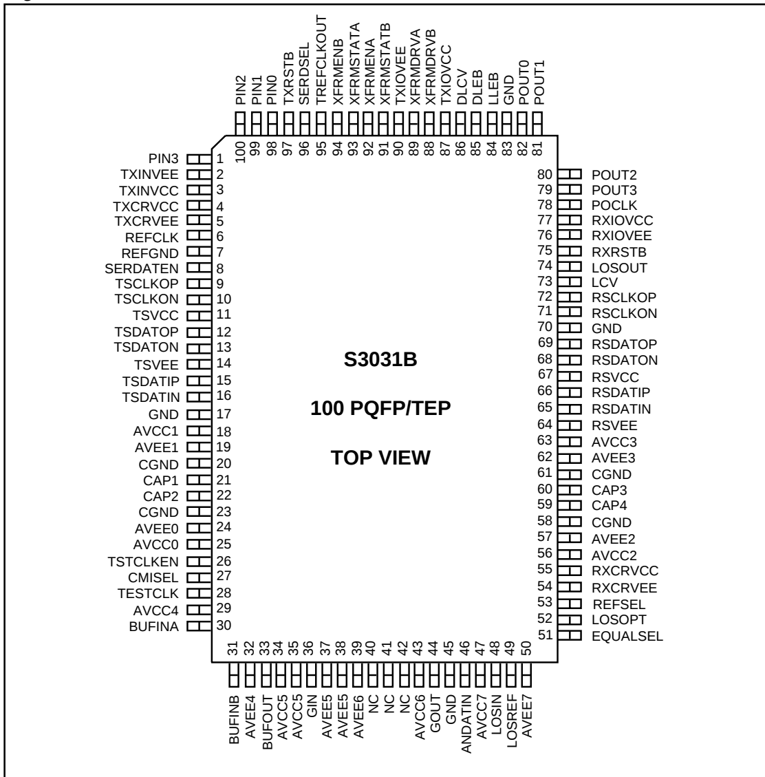
Figure 15. S3031B Pinout
