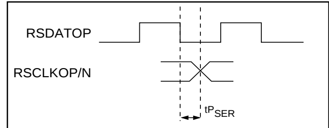
Figure 11. S3031B Clock to Data Timing
