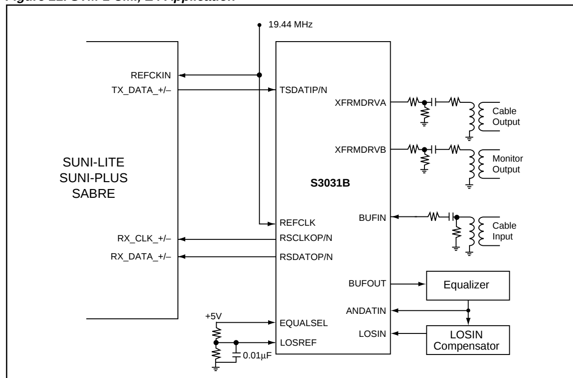
Figure 21. STM-1 CMI, E4 Application
