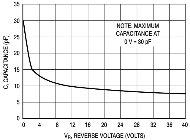
Figure 6. Maximum Capacitance
