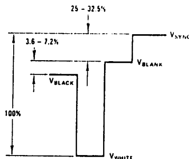
FIGURE 2. Composite Video Voltage Percentages
