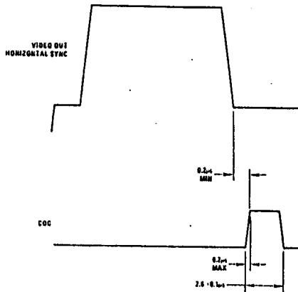
FIGURE 6. Color Gate Signal Timing
