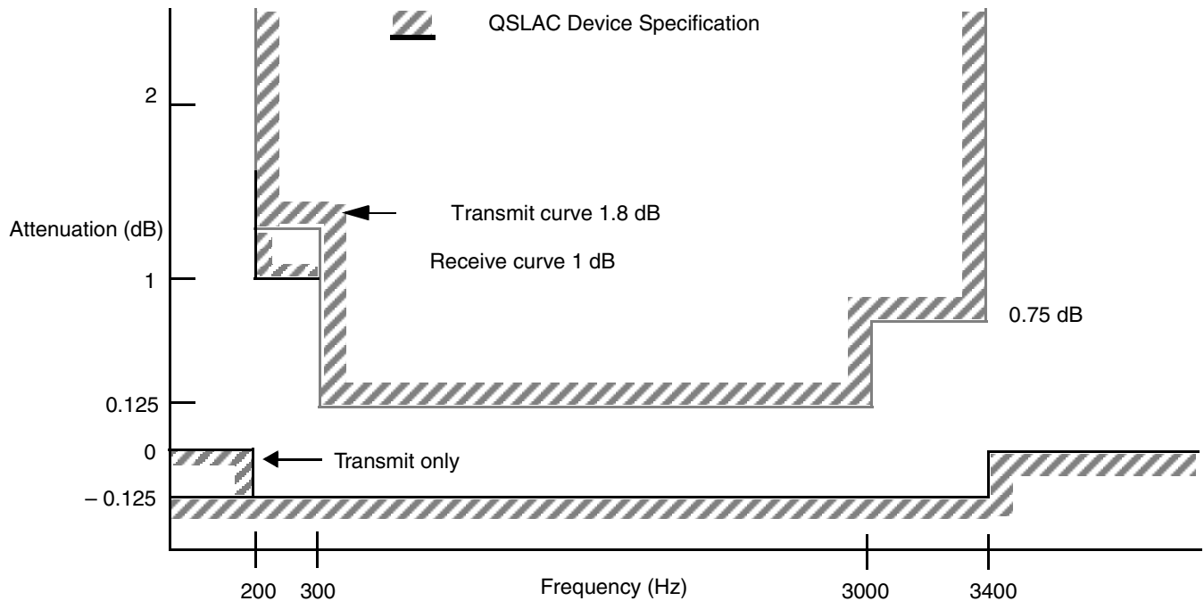
Figure 1. Attenuation Distortion
