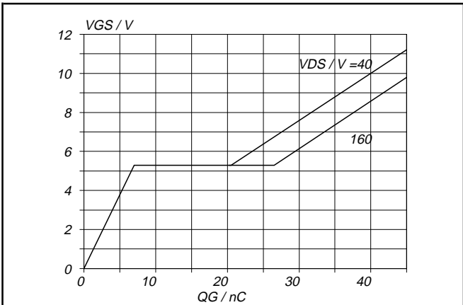
Fig.13. Typical turn-on gate-charge characteristics. V_{GS} = f(Q_G) ; conditions: I_D = 19\text{ A} ; parameter V_{DS}
