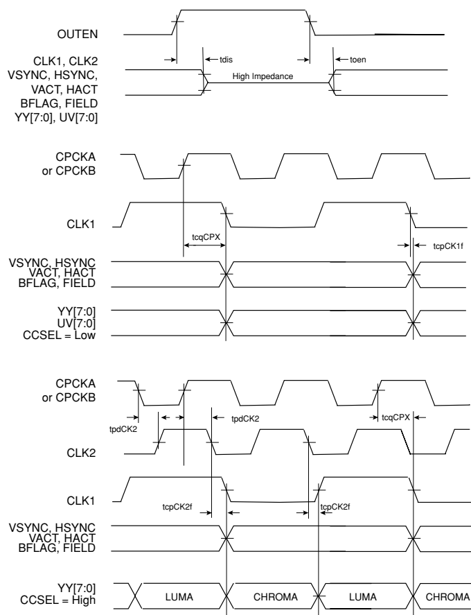
Fig.2 Video Interface Timing Diagram
