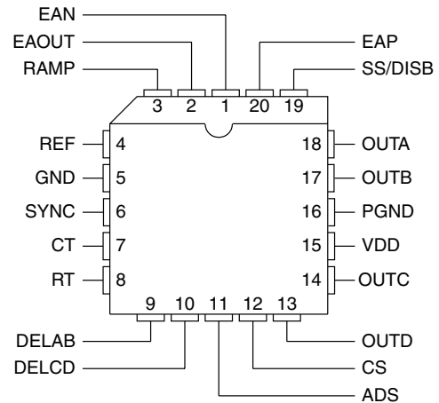
PLCC-20, CLCC-20 (TOP VIEW) Q Package, L Package
