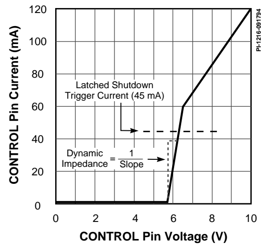
Figure 10. TOPSwitch CONTROL Pin I-V Characteristic.
