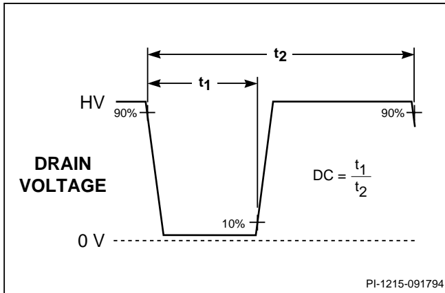
Figure 9. TOPSwitch Duty Cycle Measurement.
