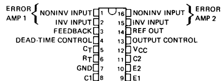
TL495C . . . N PACKAGE
