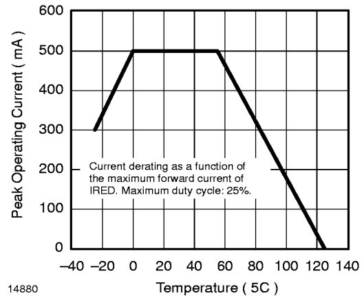
Figure 12. Current Derating Diagram
