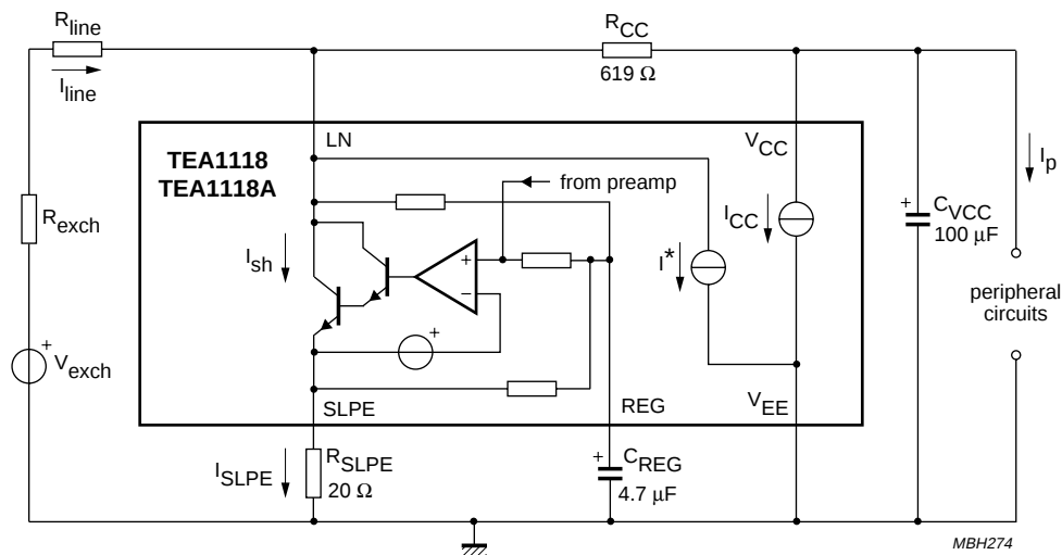
Fig.7 Supply configuration.
