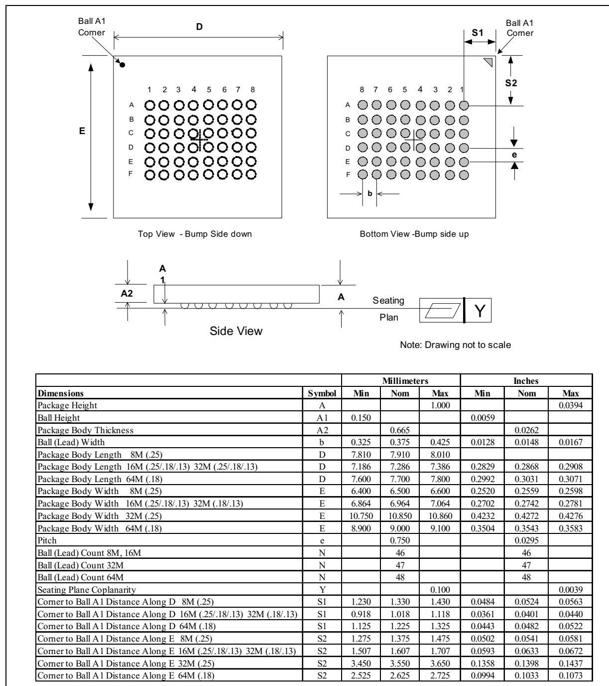
Figure 1. \mu BGA* and VF BGA Package Drawing and Dimensions
