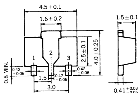
OUTLINE DIMENSIONS (Unit : mm)
