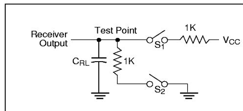
Figure 2. Receiver Timing Test Load Circuit
