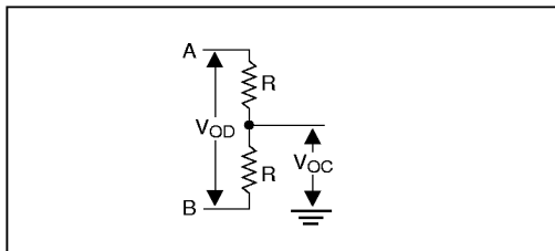
Figure 1. Driver DC Test Load Circuit
