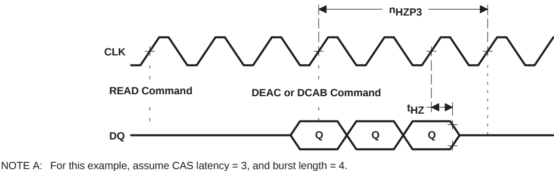
Figure 22. Read Followed by Deactivate
