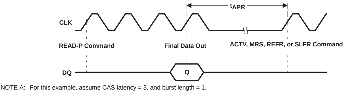
Figure 23. Read With Auto-Deactivate
