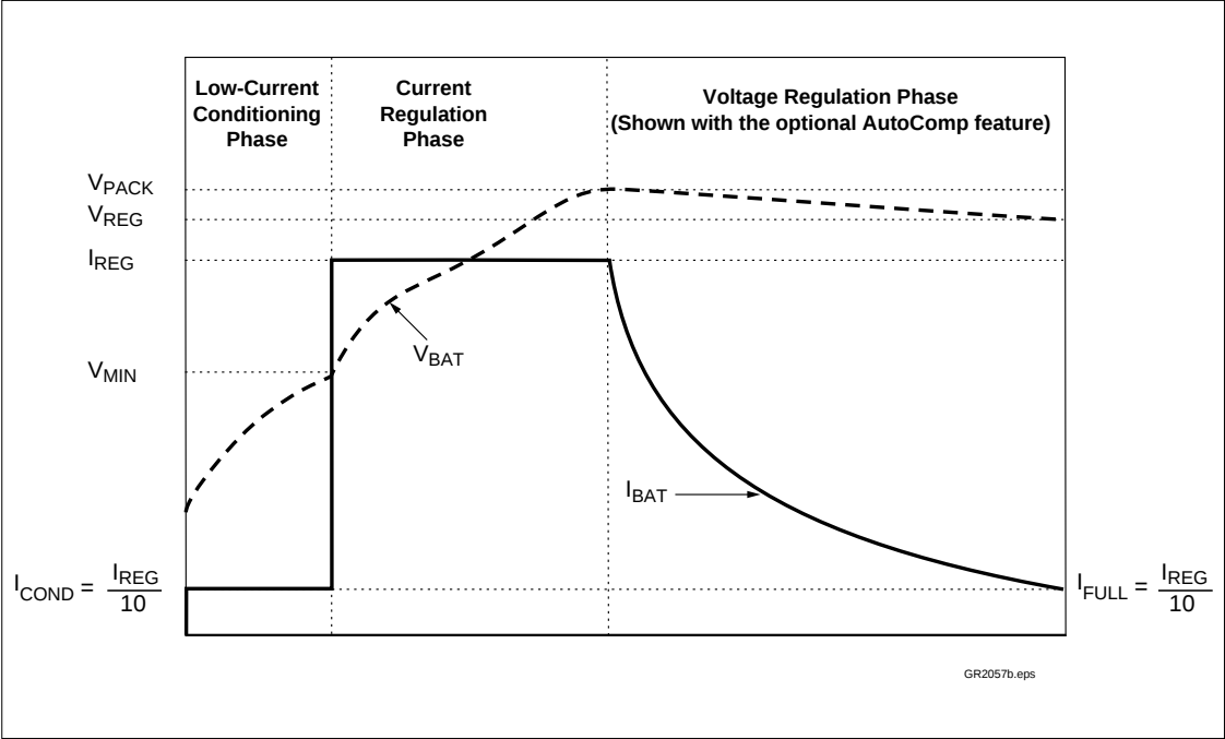
Figure 4. Typical Charge Algorithm
