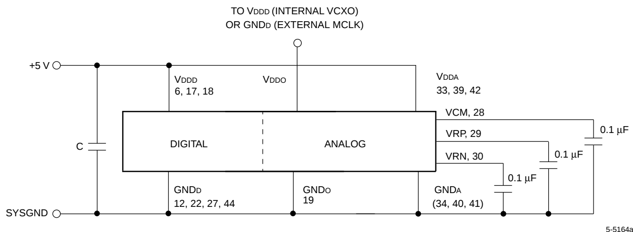
Figure 5. Recommended Power Supply Connections
