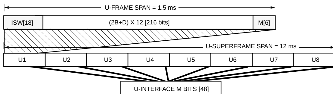
Figure 12. U-Interface Frame and Superframe
