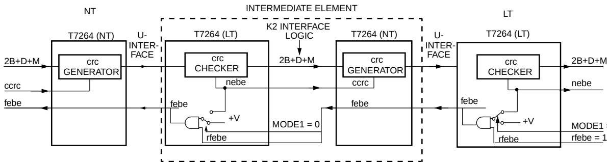
Figure 20. Use of rfebe in a Multilink Configuration
