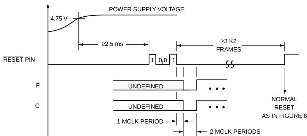
Figure 7. \overline{\text{RESET}} Timing for Synchronized Clocks
