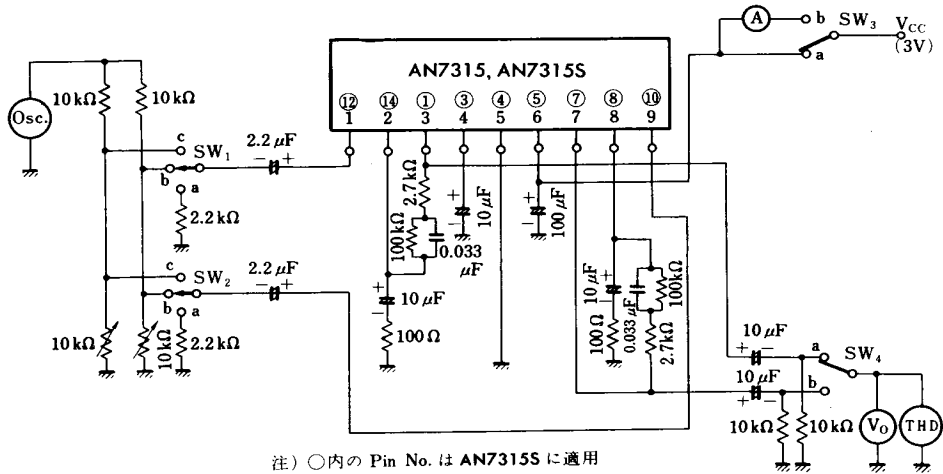
Test Circuit 1
