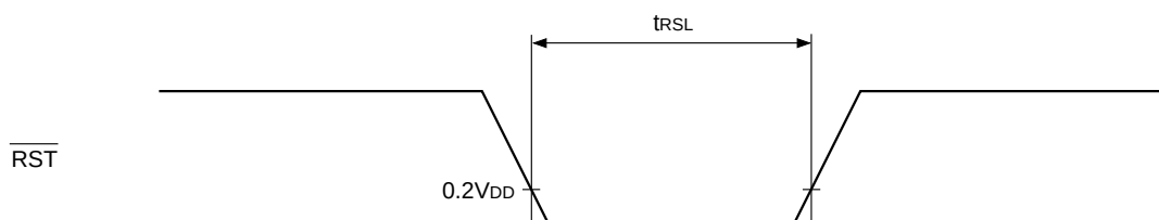
Fig. 6. \overline{\text{RST}} input timing
