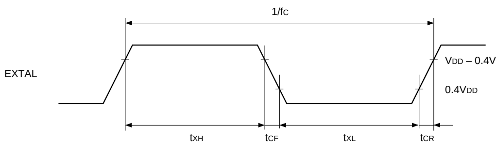
Fig. 1. Clock timing
