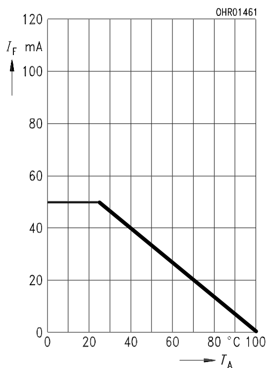
Maximum permissible forward current I_F = f(T_A) , R_{\text{thJA}} = 450 \text{ K/W}
