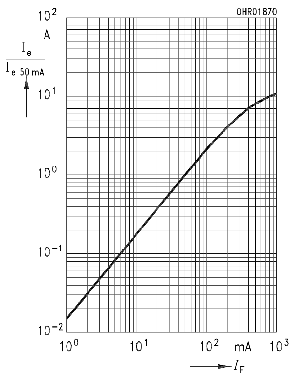
Relative output power I_e/I_{e(50 \text{ mA})} = f(I_F) single pulse, duration = 20 \mu\text{s}
